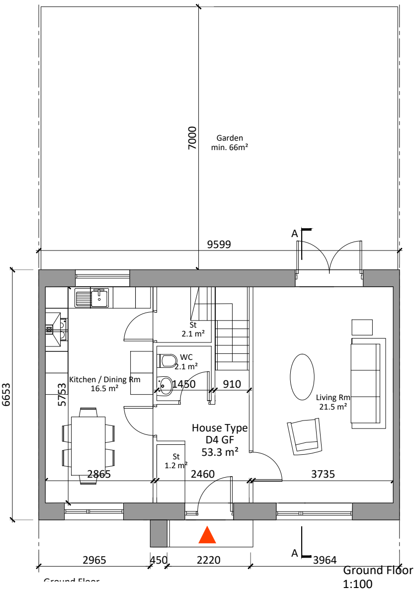
House Type D4 - Plans, Section, Elevations
